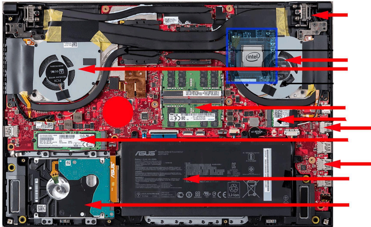
Laptop internal components with name
